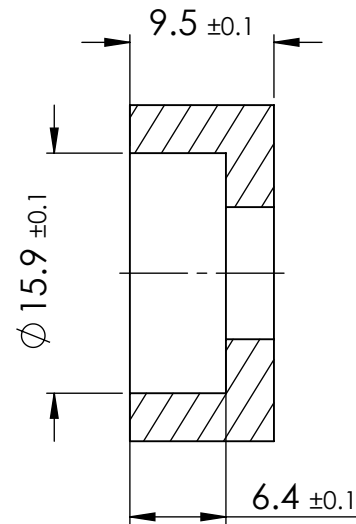
SECTION Y-Y
